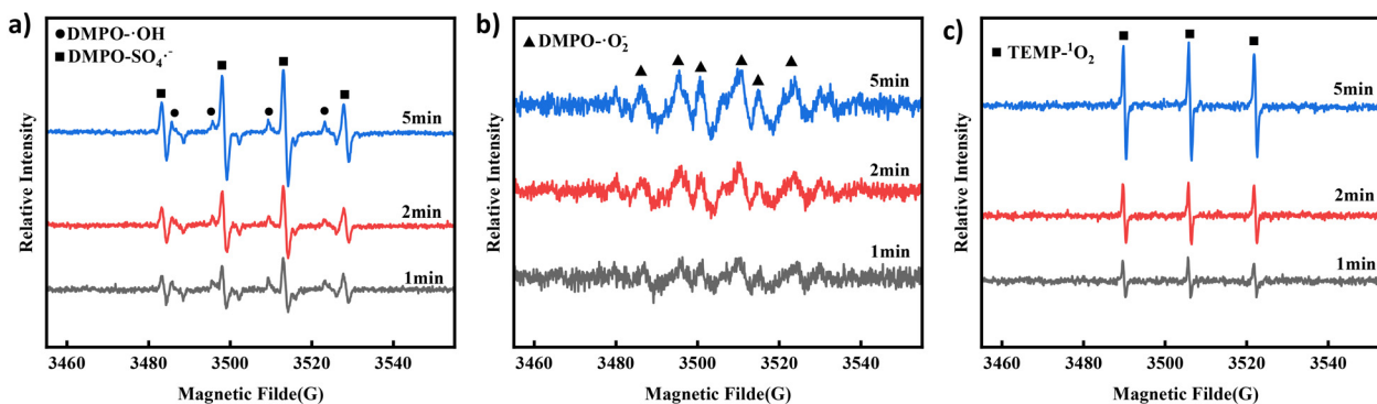
Fig. 4 EPR spectra of (a) DMPO· \text{OH} and DMPO· \text{SO}_4^{\cdot-} , (b) DMPO· \text{O}_2^{\cdot-} and (c) TEMP· ^1\text{O}_2 at different reaction times in the Co NP-PBC/PMS/TCH system.
