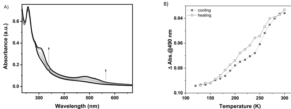
Fig. 4 (A) Evolution of the UV-visible absorption spectra of a 1-Pt film ( N = 20 cycles, T = 253 \text{ K} , c = 50 \text{ mM} ) recorded upon cooling from 300 K to 100 K. (B) Temperature dependence of the absorbance band intensity at 490 nm.
