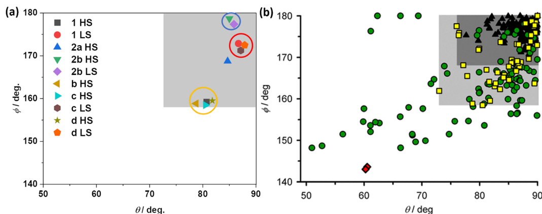
Fig. 10 Angular parameters of HS and LS states of iron(II)-BPP complexes. (a) Angular parameters of HS and LS forms of complexes 1\text{-CH}_3\text{CN} , b , c , and d , and 2\mathbf{b}\text{-CH}_3\text{CN}\text{-Y} . For complexes b and 2a only HS structures are available, and the angular parameters obtained from the structures are shown. (b) A compilation of angular parameters reported for iron(II)-BPP complexes. (b) is reproduced from the study by Halcrow and co-workers. 37 Copyright © 2024 The authors. Open access licensed under CC-BY 4.0.
