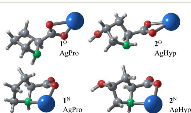
Fig. 9 Two different optimized structure types predicted for the complexes AgPro and AgHyp in solution state (B3LYP/3-21G, CPCM, water). 76
