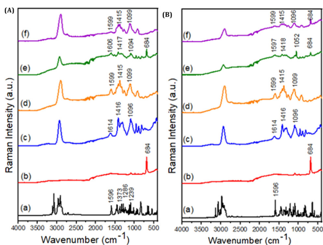
Fig. 3 Raman spectra for: (A) – (a) TD; (b) LAP; (c) ALG; (d) CMC; (e) ALG2-LAP2-TD; and (f) CMC2-LAP2-TD and (B) – (a) TB; (b) LAP; (c) ALG; (d) CMC; (e) ALG2-LAP2-TB; and (f) CMC2-LAP2-TB. The membrane codes are described in Table 1.
