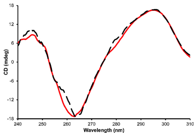
Fig. 6 CD spectrum of 5.65 \mu\text{M} HTS (black broken line) and in the presence of 37.36 \mu\text{M} of 2 (red line) in PBS buffer, pH 7.41 at 25 ^{\circ}\text{C} .
