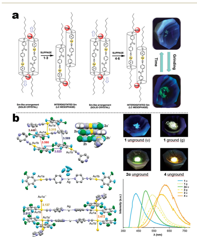
Fig. 17 (a) Schematic illustration of spacer-dependent solid-assembly model of complexes 5-4. Reproduced from ref. 113 with permission. Copyright (2022), The Royal Society of Chemistry. (b) Crystal structure and Au...Au interaction of complex 5-6B. Reproduced from ref. 114 with permission. Copyright (2019), The Royal Society of Chemistry.
