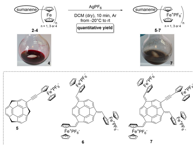
Fig. 4 Oxidation of the sumanene-ferrocene conjugates 2 – 4 to \text{Fc}^+ -containing compounds 5 – 7 . Solution colours before and after the reaction in the representative synthesis of 7 from 4 are also presented.
