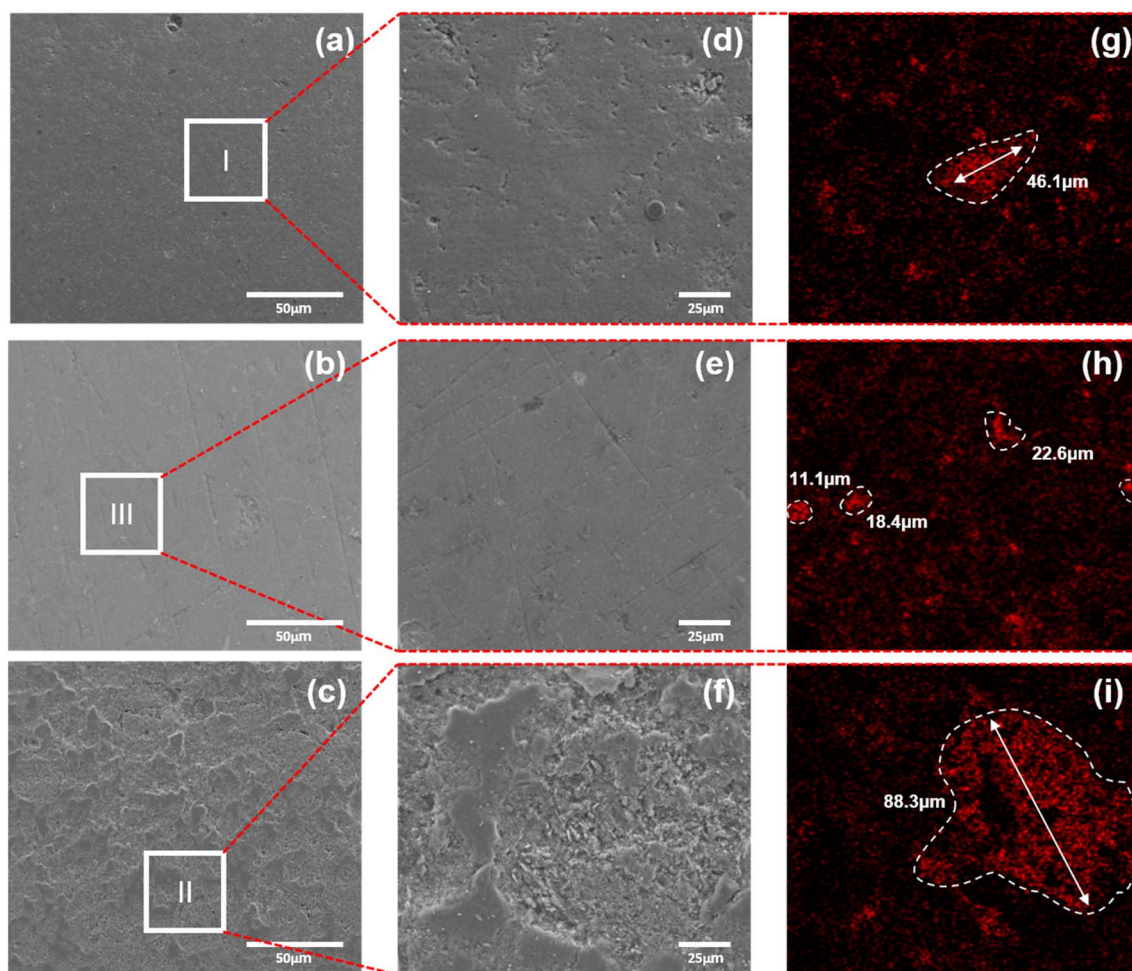
Fig. 7 (a–f) Cross-sectional images and (g–i) EDS analysis of geopolymers: (I) GP OFC , (II) GP OFC and (III) GP OC . (a–c) and (d–f) show surfaces at different magnifications. In (g–i), Ca elements are indicated in red, and the size of Ca compounds is estimated.
