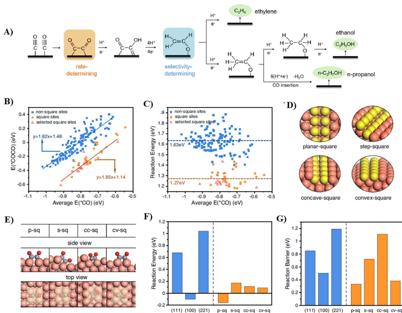
Fig. 23 Identification of C–C coupling active sites: (A) reaction pathway for C 2+ products in CO 2 reduction; (B) adsorption energy of *COCO as a function of the average adsorption energy of two adsorbed *CO; (C) reaction energy (2*CO → *COCO) as a function of the average E(*CO) on these sites; (D) DFT periodic slab configurations of four square-like sites; (E) *OCCO configurations on these four sites (solvent molecules have been removed to show the adsorbate configurations); (F) reaction energies, and (G) barriers (2*CO → *COCO) on different DFT slab models under appropriate electrochemical interface. Color code: brown-Cu; yellow-Cu in square-like sites; gray-C; and red-O. 37
