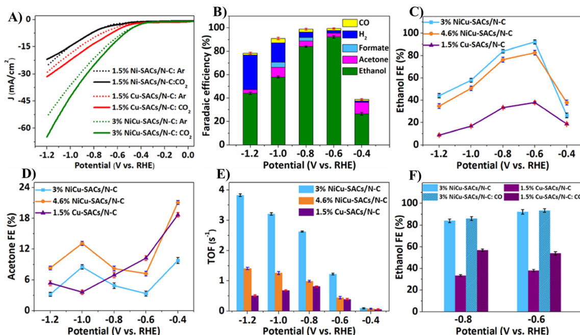
Fig. 26 (A) LSV curves of 3% NiCu-SACs/N in 0.5 M KHCO 3 . (B) FE% & product distribution on 3% NiCu-SACs/N-C. (C) FE% of ethanol, (D) FE% of acetone, and (E) TOF of ethanol over NiCu-SACs/N-C hybrids with different metal loadings at different applied potentials. (F) FE% of ethanol over 3% NiCu-SACs/N-C and 1.5% Cu-SACs/N-C. Reproduced with permission. 236 ©2024, Elsevier B.V.
