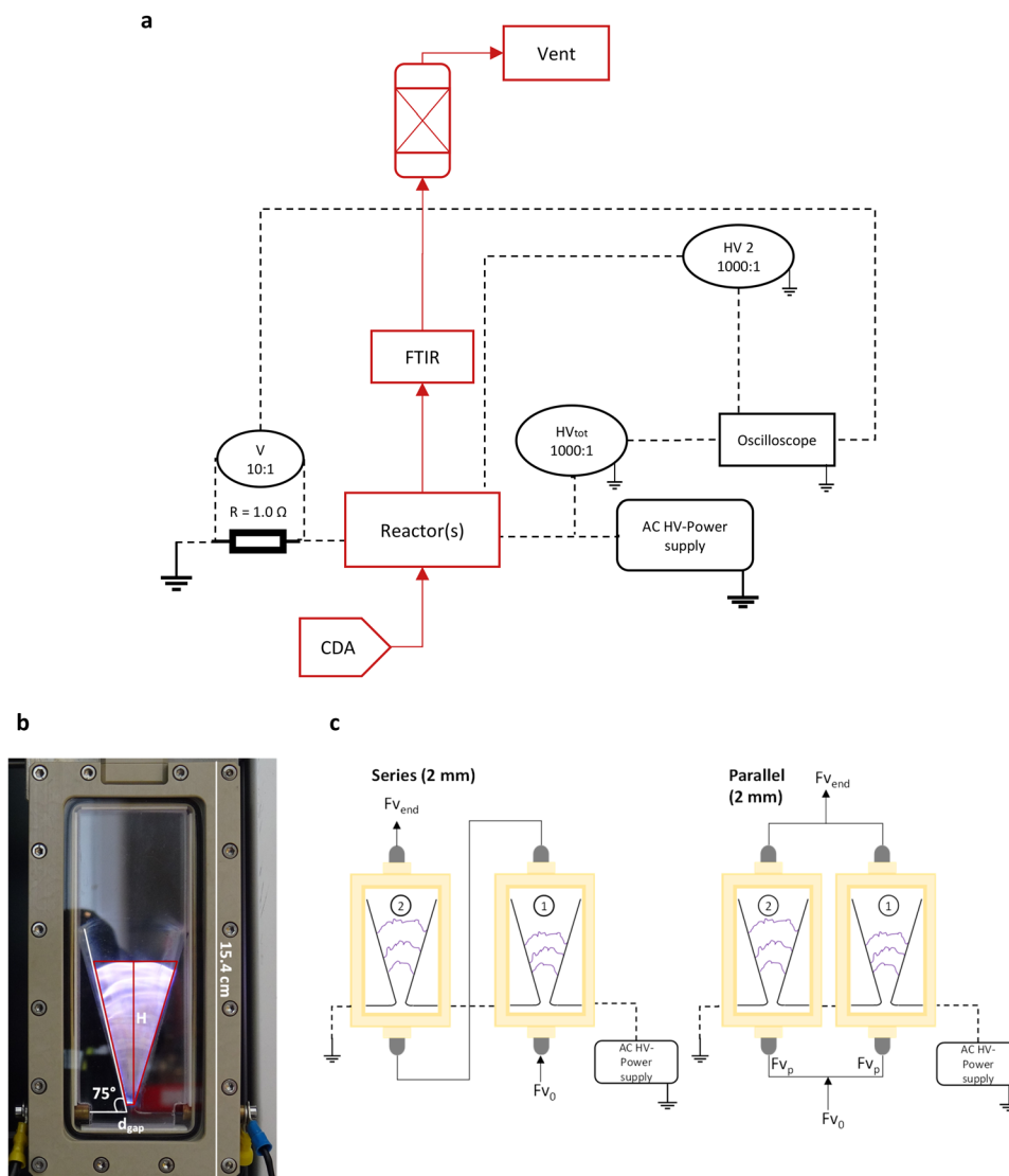
Fig. 1 (a) Experimental set-up schematic. (b) A single GEAR with a 2 mm discharge gap. The trapezoid surface in red represents the plasma volume at a flow rate of 1 L min -1 CDA. (c) Schematics of the series and parallel topology, including gas (solid) and electrical (dashed) connections.
