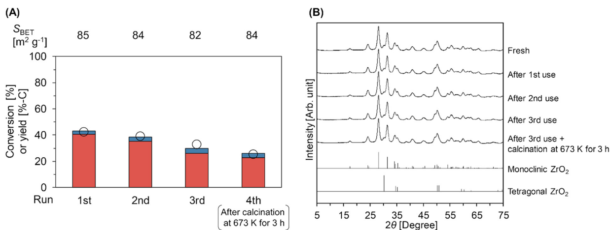
Fig. 3 (A) Reuse test of the m-ZrO 2 catalyst in Gly-Gly hydrolysis and (B) XRD patterns of fresh and spent m-ZrO 2 catalysts. Legends for fig. A: white circles = conversion of Gly-Gly; red bars = yield of glycine; blue bars = yield of glycine anhydride. Reaction conditions: Gly-Gly 2.0 mmol; m-ZrO 2 (calcined at 673 K) 0.10 g; H 2 O 5.0 g; 353 K; 4 h. The m-ZrO 2 catalyst was reused after washing with water and drying through the 1st to 3rd run, while the 4th run was operated after the calcination of the spent catalyst in air at 673 K for 3 h. The detailed data are shown in Table S8.† References for fig. B: monoclinic ZrO 2 = ICSD card #18190; tetragonal ZrO 2 = ICSD card #68781.
