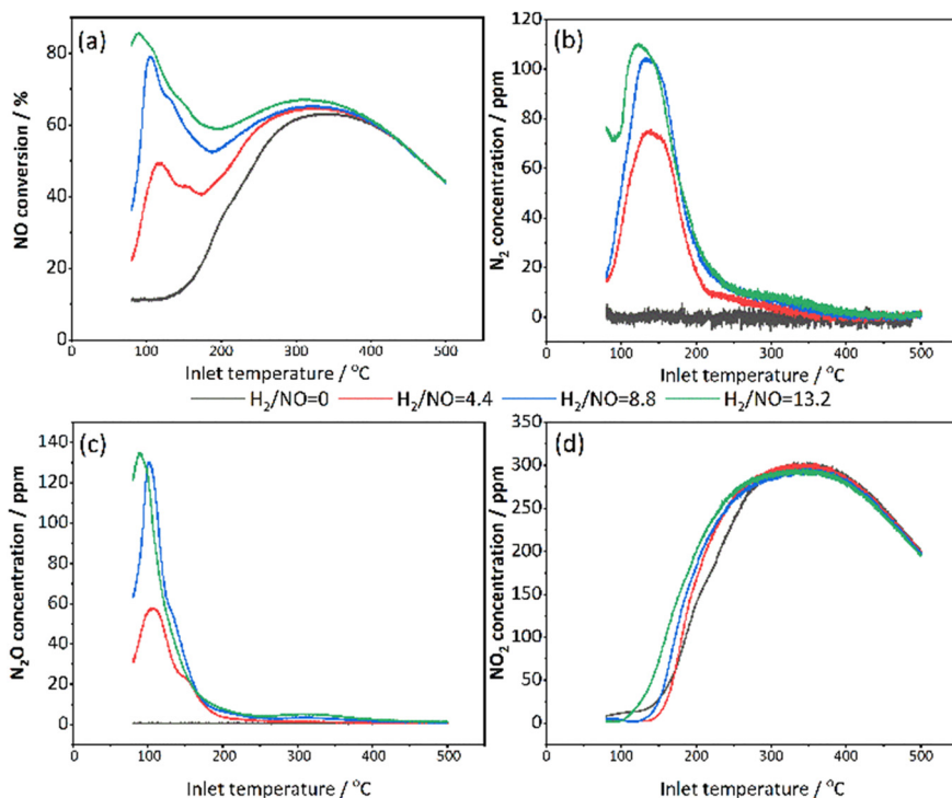
Fig. 7 Comparison of the effect of \text{H}_2/\text{NO} ratios on 2 wt% Pt/SSZ-13 catalyst, where (a) shows the conversion, and the concentration profiles are shown in (b) \text{N}_2 (c) \text{N}_2\text{O} (d) \text{NO}_2 (GHSV = 20 000 \text{h}^{-1} (STP); gas inlet: 10% \text{O}_2 , 5% \text{H}_2\text{O} , 500 ppm NO, 2200/4400/6600 ppm \text{H}_2 balanced in Ar; T : 80–500 ^\circ\text{C} ; heating rate: 5 ^\circ\text{C min}^{-1} ).
