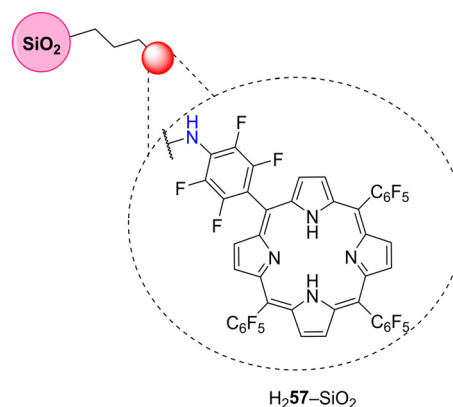
Fig. 26 Representation of the H_257 -silica photocatalyst (more para -atoms may be substituted).
