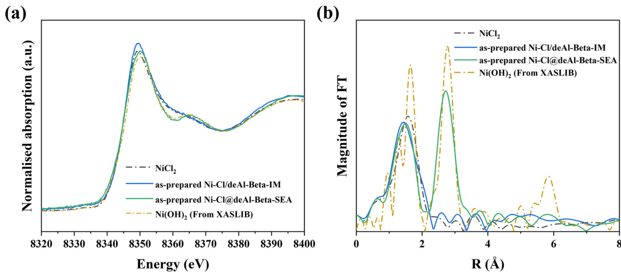
Fig. 3 Ni K-edge XANES analysis (a) of Ni form in as-prepared Ni-Cl/deAl-beta-IM and Ni-Cl@deAl-beta-SEA (after drying at 120 °C for 4 h) and (b) the Fourier transform of k^3 -weighted EXAFS spectra.
