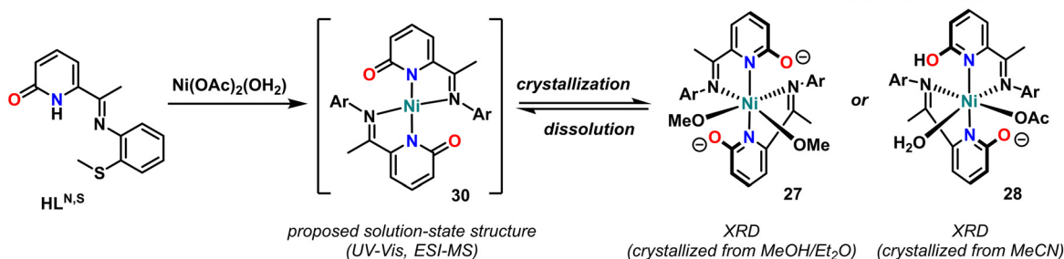
Scheme 11 Selected examples of molecular nickel pyridonate complexes (top). Acceptorless alcohol dehydrogenation catalyzed by 26 (center). Solution and solid-state structures of nickel pyridonates 27 , 28 , and 30 (bottom).
