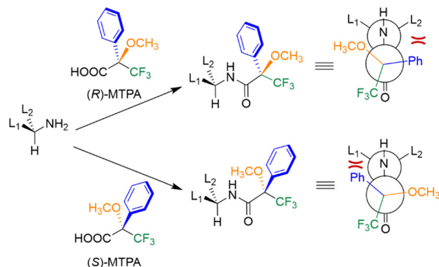
Fig. 13 NMR analysis of a chiral amine through derivatization with Mosher acid. The different shielding of the \text{L}_1 and \text{L}_2 groups of the amine are highlighted in red. Depending on the enantiomer of MTPA acid employed, different shielding effects on the \text{L}_1 and \text{L}_2 groups of the amine are observed.
