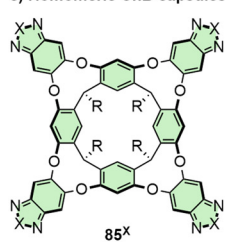
Fig. 17 Halogen- and chalcogen-bond interactions, including with halonium ions, can be used to assemble both homo- and heteromeric capsules. R groups omitted from SCXRD structures for clarity.
