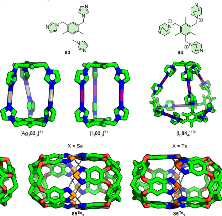
Fig. 17 Halogen- and chalcogen-bond interactions, including with halonium ions, can be used to assemble both homo- and heteromeric capsules. R groups omitted from SCXRD structures for clarity.
