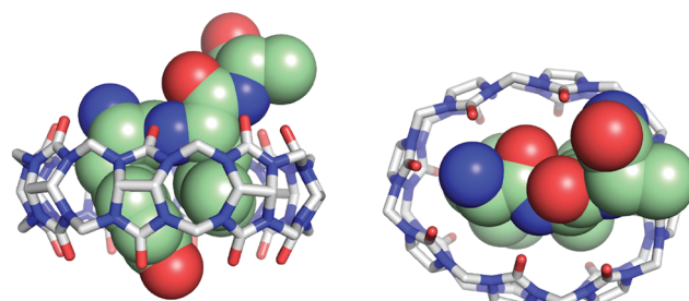
Fig. 11 (top) Relative change in fluorescence of 1:1:1 peptide:Q8:MBBI relative to Q8-MBBI under the same condition. 60 The peptide sequences are H-Tyr-Var 1 -Ala-NH 2 and H-Tyr-Ala-Var 2 -NH 2 . Reproduced with permission from ref. 60. Copyright 2015 American Chemical Society. (bottom) Rendering of the semiempirical NMR structure of the Q8-H-Tyr-Leu-Ala-NH 2 complex in two views. The peptide is shown as space-filling, and Q8 as sticks. Peptide carbons are green. Q8 carbons are grey. Oxygens are red. Nitrogens are blue. Hydrogens are not shown.
