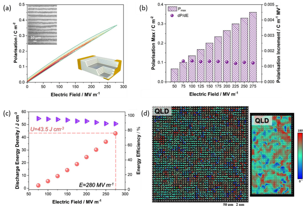
Fig. 14 QLD type MLCCs performance. (a) Unipolar P - E curves of \text{NNTa}_{0.10} -10ST-2LMT MLCCs up to the maximum field. (b) Polarisation maximum and increment as a function of electric field up to 280 \text{ MV m}^{-1} . (c) Energy storage performance up to the maximum field. (d) The [001]-oriented atomic resolution HADDF-STEM images for \text{NNTa}_{0.10} -10ST-2LMT (QLD) with the projected polarisation angle. Individual arrows show B-site cation displacement vectors in individual unit cells with different vector angles. 18 Reprinted with permission from ref. 18, the John Wiley and Sons., under the terms of the Creative Commons CC BY license.
