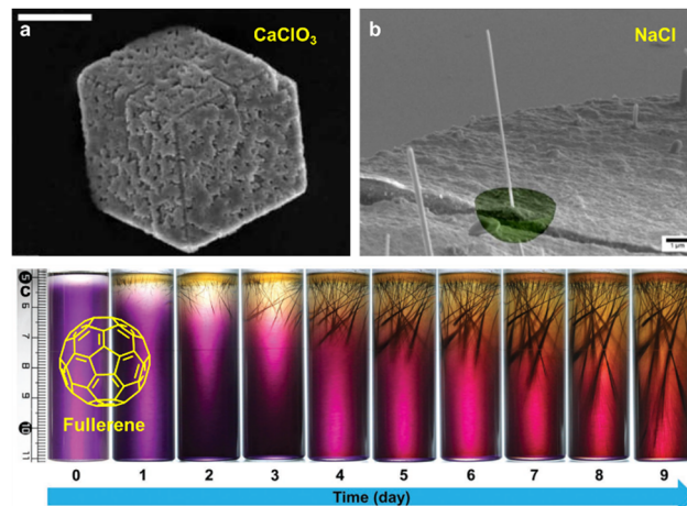
Fig. 3 (a) SEM image of a calcite crystal obtained within hydrogels of 1 after 24 h with etched surface provoked by the occlusion of the gel matrix, scale bar 20 μm (Adapted with permission from ref. 38. Copyright 2004 Royal Society of Chemistry). (b) SEM image high aspect NaCl nanowires grown on the surface of Eu 3+ cross-linked gel 2 (Adapted with permission from ref. 41. Copyright 2013 American Chemical Society). (c) Photographs of the two-layer counter-diffusion crystallization of C 60 within m -xylene gels of 3 over 9 days triggered by the addition of acetonitrile (Adapted with permission from ref. 42. Copyright 2019 John Wiley and Sons).
