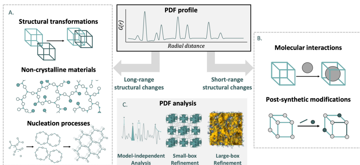
Fig. 2 Schematic view of the problems in MOF and COF chemistry that can be solved using PDF experiments divided by the type of alterations of the network: average structure alterations (A), and local-structure alterations (B). Additionally, different types of PDF analysis (C).
