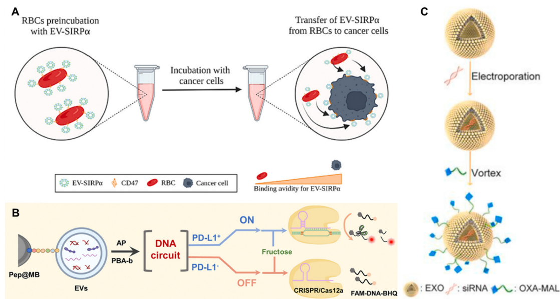
Fig. 20 Exosomes derived from other various sources. (A) EVs that express SIRPα, EV-SIRPα, is a RBC-derived exosomes that can hinder the CD47 “don’t eat me” signaling present on tumor for cancer immunotherapy. Reproduced from ref. 220 Copyright 2022 with permission from Elsevier. (B) Circulating exosomes for lung cancer diagnosis and immunotherapy response prediction. A programmable DNA circuit will translate the presence of PD-L1 into the appearance of duplex DNA probes on the surface of the EVs to activate the trans -cleavage activity of CRISPR/Cas12a system, which finally produces a significant fluorescence signal. Reproduced from ref. 265 Copyright 2023 with permission from American Chemical Society. (C) Bone marrow mesenchymal stem cell (MSC)-derived exosomes for immunotherapy of pancreatic ductal carcinoma (PDAC). The exosomes from MSCs were isolated by gradient centrifugation and loaded with galectin 9 siRNA via electroporation. The surface of the exosome was modified with oxalipatin (OXA) to trigger immunogenic cell death. Reproduced from ref. Copyright 2021 with permission from Elsevier.
