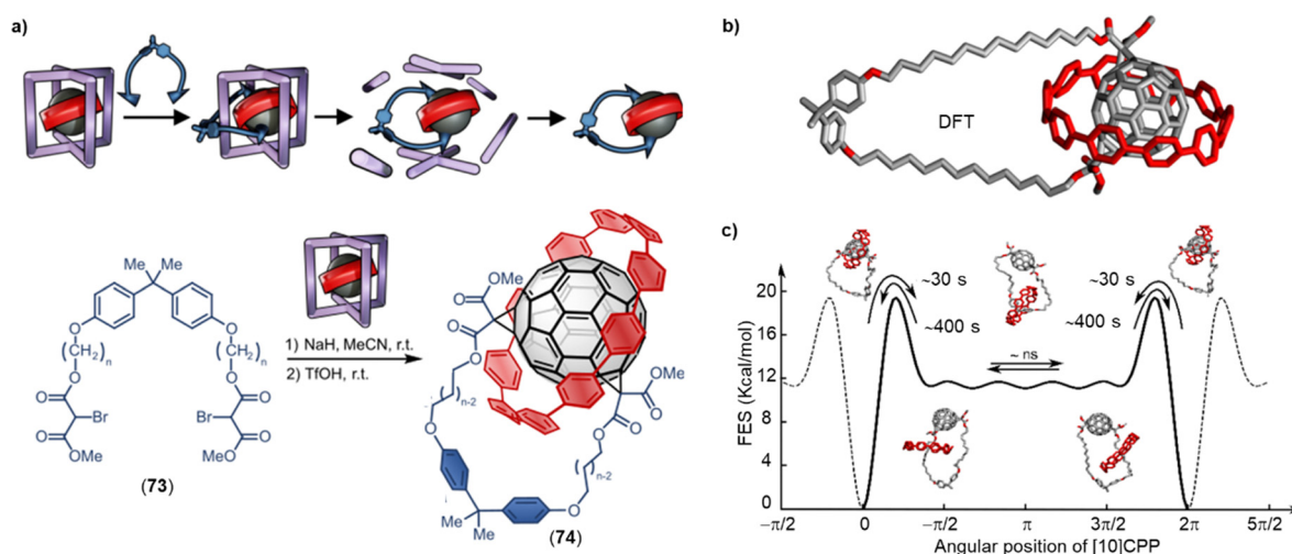
Fig. 26 (a) The synthetic strategy of C_{60} /[10]CPP-catenanes (74). (b) Atomistic molecular model of the C14- C_{60} /[10]CPP-catenane. (c) Free-energy diagram as a function of the angular position of [10]CPP along the larger ring of the catenane.
