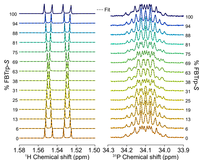
Fig. 3 ^1\text{H} (left) and ^{31}\text{P} (right) NMR spectra at 850 MHz from which \Delta_d values were extracted for the final comagnetometry plot shown in figure 4. ^1\text{H} spectra were collected using a BIRD pulse sequence (see SI) and fit with the sum of four complex Lorentzian lines with independent phase and peak center. ^{31}\text{P} spectra were acquired using a simple 90^\circ pulse sequence without ^1\text{H} decoupling and fit with a sum of two multiplets (doublet of quartets, \text{AXY}_3 spin system) with no phase, assuming purely absorptive lineshapes. Experimentally obtained spectra are overlaid with the best fit line at each sample composition.
