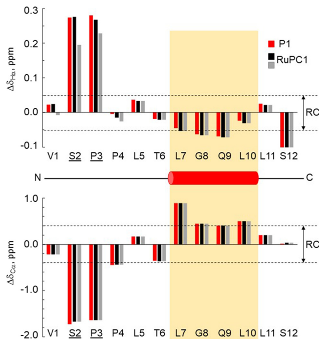
Fig. 4 Chemical shift deviations for the ^1\text{H}_\alpha protons ( \Delta\delta_\text{H}_\alpha = \delta^\text{observed}_\text{H}_\alpha - \delta^\text{RC}_\text{H}_\alpha , ppm) and ^{13}\text{C}_\alpha carbons ( \Delta\delta_\text{C}_\alpha = \delta^\text{observed}_\text{C}_\alpha - \delta^\text{RC}_\text{C}_\alpha , ppm) for the major species of P1 (red bars) and RuPC1 (black and grey bars) as a function of sequence. \delta^\text{RC}_\text{H}_\alpha and \delta^\text{RC}_\text{C}_\alpha were taken from ref. 63. Pro-preceding residues are underlined. The two dashed lines indicate the random coil range (RC). Top cartoon indicates the secondary structure; helix is shown as a red cylinder.
