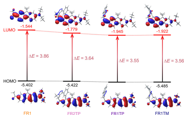
Fig. 5 Frontier molecular orbitals contour plots and energies for FR1 , FR2TP , FR1TP and FR1TM at the mPW1PW91/6-311+G(2d,p)//mPW1PW91/6-31+G(d) level (isosurface value: 0.03 a.u.). Orbital energies indicated are in eV.
