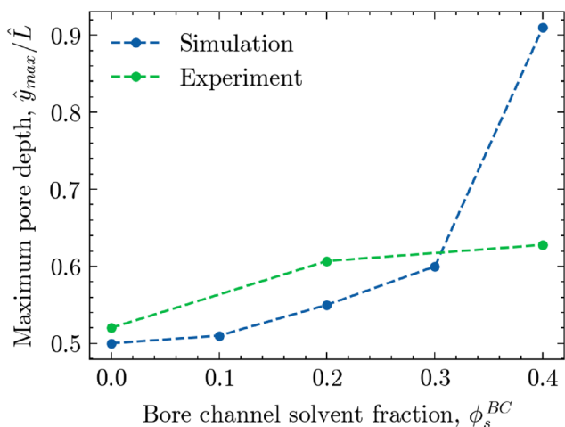
Fig. 9 The maximum pore depth \hat{y}_{\max}/\hat{L} , corresponding to the relative depth within the bijel cross-section where the pore size reaches its maximum value, versus the solvent fraction of the interior bore channel \phi_s^{BC} . The green markers correspond to experimental bijel structures, whereas the blue markers correspond to the structures provided by the phase-field model.
