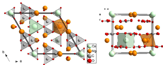
Fig. 1 Projections along the c (left) and b axes (right) of the crystalline R32 \text{Mg}_3\text{Ca}(\text{CO}_3)_4 huntite structure at room conditions. Thick black lines indicate the unit-cell. Light green, orange, light gray, and red spheres represent Ca, Mg, C, and O atoms, respectively. A [\text{CaO}_6] trigonal prism and a [\text{MgO}_6] octahedron are depicted to illustrate the different coordination sphere around the cation atoms. [\text{CO}_3] trigonal planar units are also represented.
