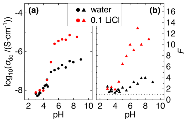
Fig. 4 (a) pH-dependent dc conductivities of PEMs and (b) pH-dependent shift factors F as derived from the scaling procedure displayed in Fig. 3. Black symbols refer to PEMs prepared in water and red symbols to those prepared in 0.1 M LiCl solution.
