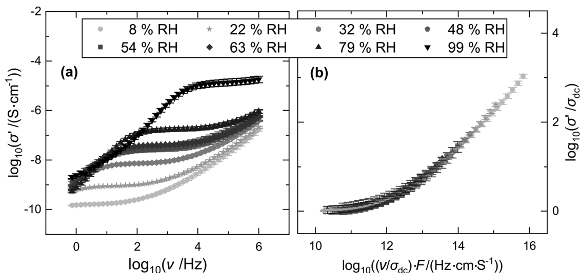
Fig. 2 Time-humidity superposition of conductivity spectra of (PDADMA/PAA) n PEMs prepared at pH 4. (a) Conductivity spectra measured at different relative humidity (RH). (b) Spectra scaled according to a time-humidity superposition.
