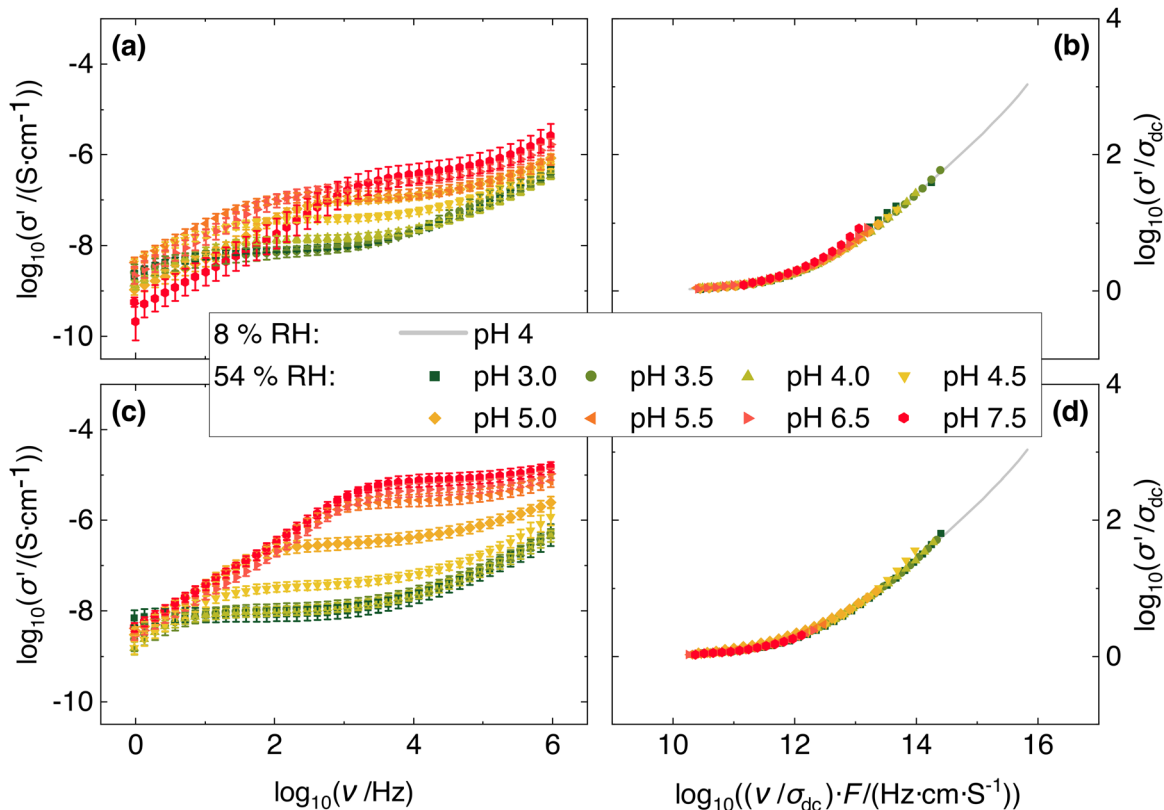
Fig. 3 Conductivity spectra of (PDADMA/PAA) n PEMs in dependence on pH and their time-pH superposition. (a) and (b) Data for samples prepared from salt-free solution adjusted to different pH values. (c) and (d) Data for samples prepared from 0.1 M LiCl solutions adjusted to different pH values. In (b) and (d) spectra obtained for different preparation pH values at constant humidity RH = 54% during the measurement are shifted with respect to the reference spectrum. Samples prepared at pH 4 and measured at 8% relative humidity are used as reference.
