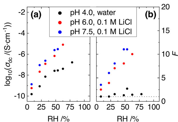
Fig. 5 (a) RH-dependent dc conductivities of PEMs and (b) RH-dependent shift factors F as derived from the scaling procedure displayed in Fig. 1. Black symbols refer to PEMs prepared at pH 4 in water, red symbols stand for PEMs prepared in 0.1 M LiCl solution at pH 6 and blue symbols for PEMs prepared in 0.1 M LiCl solution at pH 7.5.
