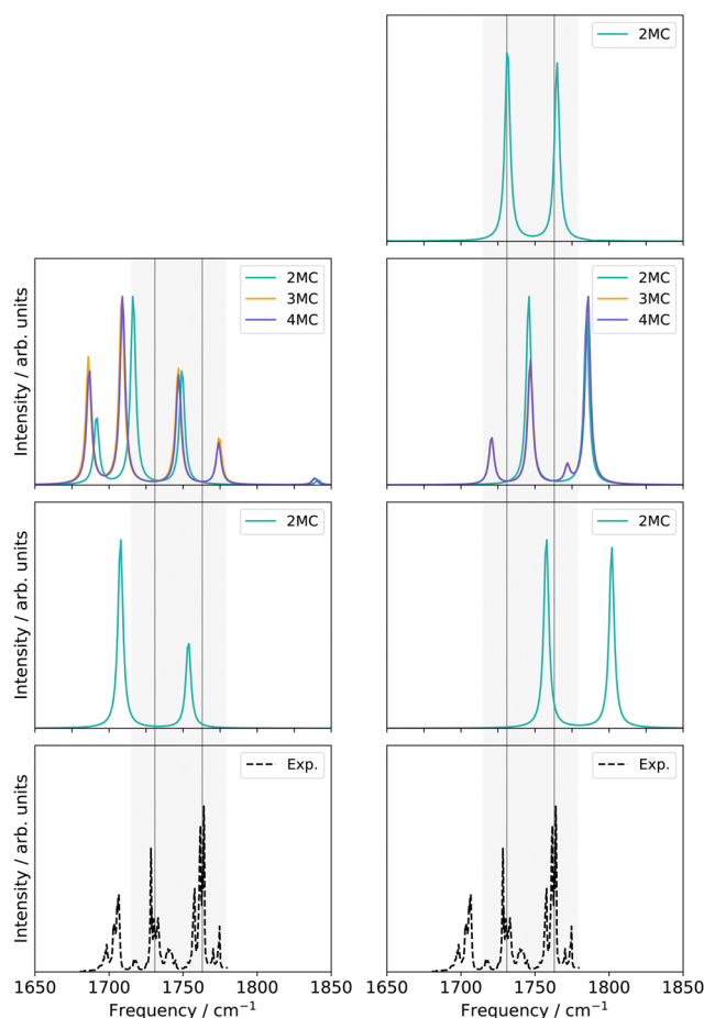
Fig. 5 Damped linear response spectra of uracil for the spectral range of 1650–1850 \text{cm}^{-1} on two-mode reduced spaces on a full coupled PES (FVCI), nine-mode reduced space on 2MC, 3MC, and 4MC property surfaces (VCC[4]), and on a 30-mode full space (VCC[2]) for FALCON and normal modes, respectively. The experiment is obtained in an Ar-matrix at T = 10 \text{ K} and taken from ref. 56. The property surfaces are calculated on the r^2 SCAN-3c level. All peak position values for the calculations can be found in the ESI† in Table SIII.
