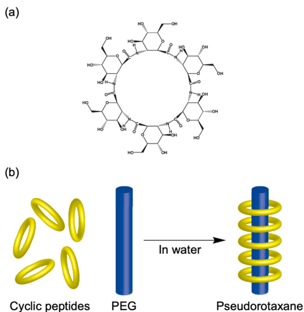
Fig. 13 (a) Chemical structures of cyclic hexamers of \beta -glucosaminic acid. (b) Schematic illustration of polypseudorotaxane formation from cyclic hexamers of \beta -glucosaminic acid and poly(ethylene glycol).
