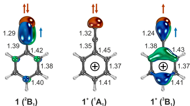
Fig. 4 Geometry and occupied \sigma and \pi orbitals of the lowest-energy states of radical 1 and singlet and triplet cation 1 + , optimized at the NEVP22/aug-cc-pVTZ level of theory. Selected C–C bond distances in Å are shown.
