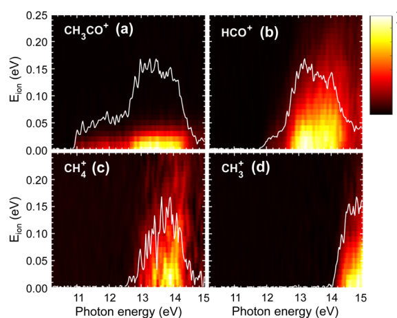
Fig. 5 Ion signal correlated to threshold photoelectrons as a function of ion kinetic energy, E_{\text{ion}} and photon energy for (a) \text{CH}_3\text{CO}^+ , (b) \text{HCO}^+ , (c) \text{CH}_4^+ , and (d) \text{CH}_3^+ . The photon energy axis corresponds to the ionization energy since only threshold electrons are considered. The TPES obtained for E_{\text{ion}} below 25 meV is plotted as white curves. The color bar on the right represents the intensity (in arb. units).
