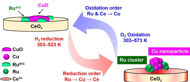
Fig. 5 Suggested structural transformation of the reversible low-temperature redox cycle of \text{Cu}_{0.18}\text{Ru}_{0.05}\text{CeO}_2 .
