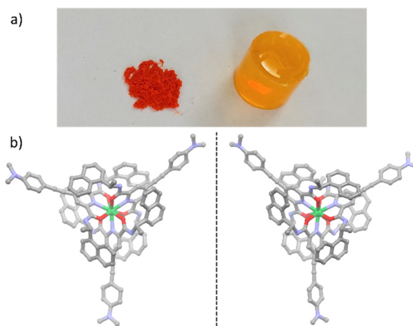
Fig. 1 (a) Pure powder of Yb(III) complex, on the left, and solution in PDMS polymer, on the right; (b) X-ray structures of [\text{Yb}(S,S\text{-L}^{\text{NHex}_2})_3(\text{OTf})_3]/\Delta\text{-Yb} (left) and [\text{Yb}(R,R\text{-L}^{\text{NHex}_2})_3(\text{OTf})_3]/\Lambda\text{-Yb} (right). Hexyl chains are simplified; hydrogen atoms, solvent molecules and OTf-anions are omitted for clarity. Green, Yb; red, O; blue, N and grey, C.
