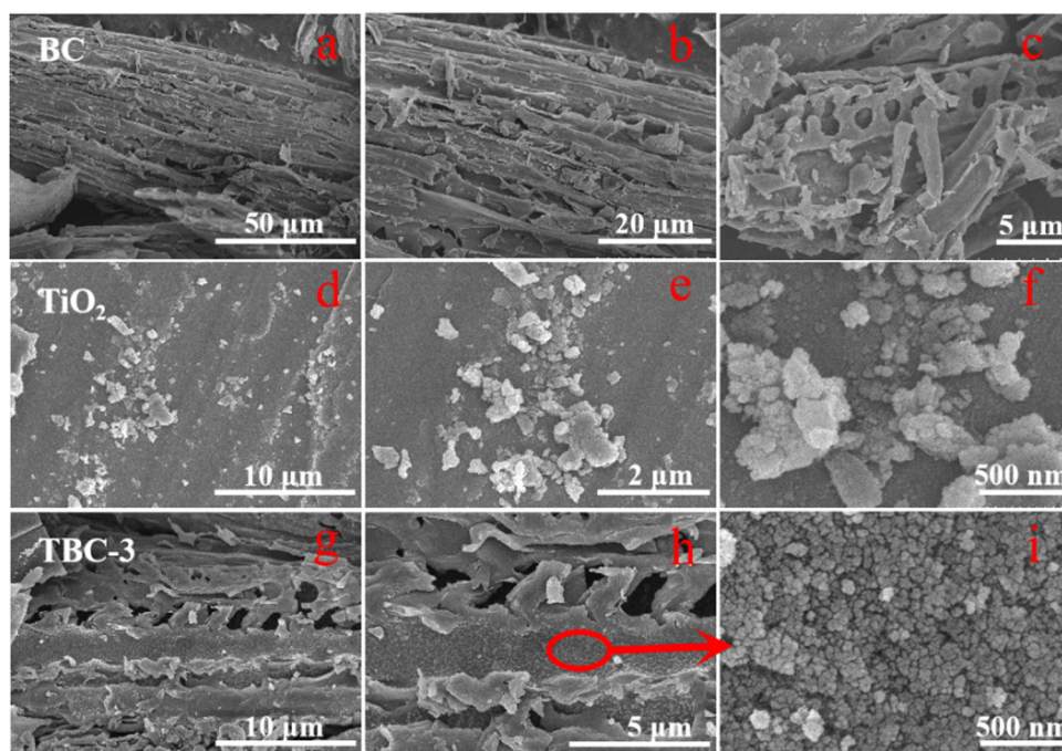
Fig. 4 Typical SEM images of the as-prepared samples. SEM images of BC (a)–(c), \text{TiO}_2 (d)–(f) and TBC-3 (g)–(i).
