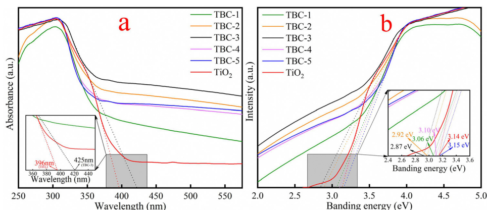
Fig. 3 UV-Vis absorption spectra (a) and corresponding band gap energies (b) of \text{TiO}_2 and TBC samples.
