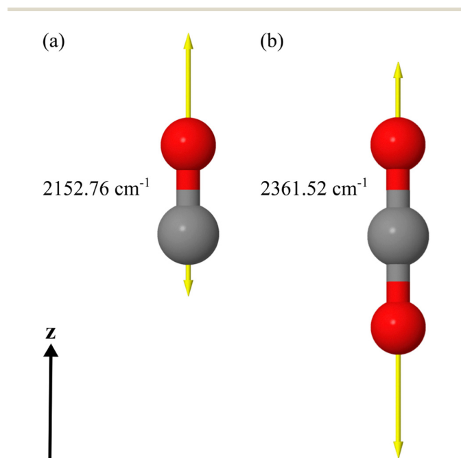
Fig. 1 (a) DFT optimized CO molecule with the displacement vector of the stretching vibrational mode at 2152.76 cm -1 . The calculated vibrational wavenumber was scaled by 0.962 to match the experimental value. The molecule is oriented along the z -axis in the calculation. (b) DFT optimized CO 2 molecule with the displacement vector of the anti-symmetric stretch vibrational mode at 2361.52 cm -1 . The calculated vibrational wavenumber was scaled by 0.962 to match the experimental value. The molecule is oriented along the z -axis in the calculation.
