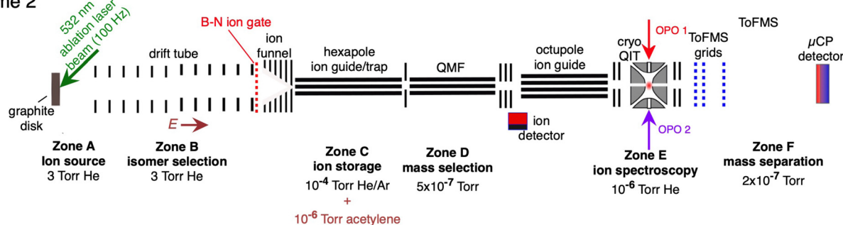
Fig. 1 IMMS-cryotrap instrument for obtaining electronic spectra of \text{HC}_{2n+1}\text{H}^+ chains. \text{HC}_{2n+1}\text{H}^+ chains were formed in two different ways. Scheme 1: \text{HC}_{2n+1}\text{H}^+ chains were produced by exposing pyrene vapour ( P \approx 5 \times 10^{-6} torr) to pulsed 266 nm radiation, which induced ionization and fragmentation. Following formation, the ions passed through an ion mobility drift tube, which served to separate different isomers. At the end of the drift tube there is a Bradbury–Nielsen (B–N) ion gate that could be used to select a particular isomer. Ions were then accumulated in a hexapole ion guide. Following ejection from the hexapole, the ions passed through a quadrupole mass filter (QMF), and an octupole ion guide, before being trapped in a cryogenically cooled quadrupole ion trap (QIT). In the QIT the ions were exposed to tunable light from an OPO overlapped (spatially and temporally) with a fixed wavelength beam from a second OPO. Resulting photofragments were separated and detected using a time-of-flight mass spectrometer. Scheme 2: \text{HC}_{2n+1}\text{H}^+ chains were produced by reacting carbon chains ( \text{C}_n^+ ), formed through laser ablation of a graphite disk, with acetylene gas at a partial pressure of \approx 2 \times 10^{-6} torr in the hexapole ion guide for \approx 0.5 s. If required, the reactant \text{C}_n^+ ions could be mobility-selected in the drift tube using the B–N ion gate. Following their creation in the hexapole, the \text{HC}_{2n+1}\text{H}^+ ions were mass-selected and spectroscopically probed in the QIT as described for Scheme 1.
