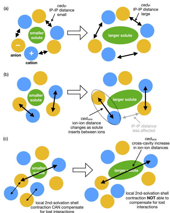
Fig. 9 Cartoons representing conceptual differences between (a) ced_{\text{IP}} and (b) ced_{\text{ions}} , and (c) representing second shell solvation effects.
