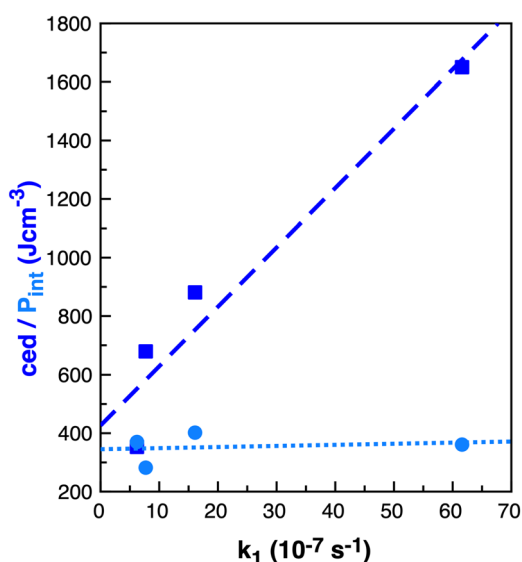
Fig. 8 Properties ced ( \text{J cm}^{-3} ) dark blue squares and P_{\text{int}} ( \text{J cm}^{-3} ) light blue circles relative to k_1 ( 10^{-7}\text{ s}^{-1} ) 25 in benzene, ethanol, acetonitrile and [\text{C}_4\text{C}_1\text{im}][\text{NTf}_2] for reaction B .
