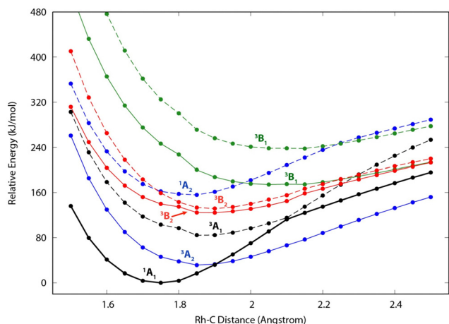
Fig. 5 Constrained potential energy curves along the metal–carbon distance in \text{RhCH}_2^+ in \text{C}_{2v} symmetry, as calculated at the EOM-SF-CCSD/cc-pVTZ-PP level of theory. Solid (dashed) lines depict the lowest-energy (first excited) state of each symmetry. The structure was optimized in the lowest state of \text{A}_1 symmetry, and all other state energies represent vertical excitations at the same structure. Spin and symmetry labels for each state, corresponding to the assignments at the ^1\text{A}_1 minimum geometry, are provided for each curve. [The symmetry labels for the \text{B}_1 and \text{B}_2 states are reversed from the Q-Chem outputs, in order to align with the symmetry-axis conventions of Gaussian computations in the remainder of this work.]
