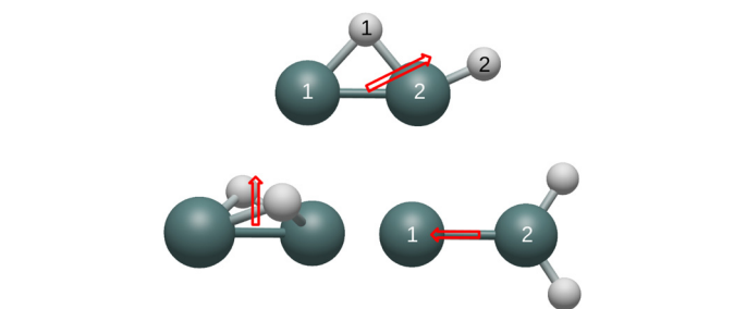
Fig. 3 Dipole moments originating from the center of mass of the cationic structures are displayed.
