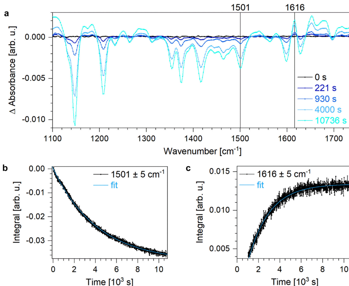
Fig. 6 (a) Changes in IR absorption upon linear-to-closed switching of DASA in toluene- d_8 at room temperature. IR absorption bands related to the linear species, e.g. at (b) 1501\text{ cm}^{-1} , disappear while new absorption bands of the closed isomers C and C', e.g. at (c) 1616\text{ cm}^{-1} , emerge.
