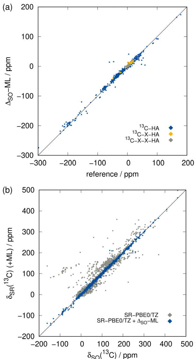
Fig. 4 Comparison of the ML-predicted SO contributions to the reference (SR/SO)-ZORA-PBE0/TZ2P ones for the ^{13}\text{C} NMR test set. (a) Values of \Delta_{SO}\delta , color-coded according to their distance to the next heavy atom (see Fig. 3(a)). (b) Total chemical shift \delta neglecting SO coupling (gray) and adding the ML-predicted \Delta_{SO}\delta (blue).
