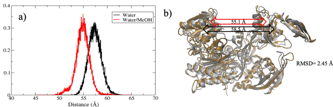
Fig. 5 (a) Distribution of PAZ-MID center of mass distance in water (black line) and water/MeOH (red line). (b) Superposition of hAgo2 middle cluster structures in water (ochre) and in water/MeOH (silver). PAZ-MID center-of-mass distance in water and water/MeOH is indicated by the black and red double arrows, respectively, inside the figure.
