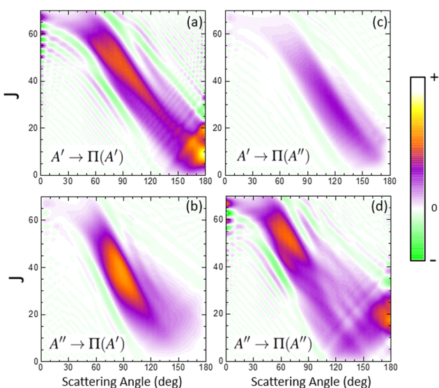
Fig. 6 Generalized quantum deflection functions (GDF) for the contribution of {}^3A' and {}^3A'' PESs to \Pi(A') and \Pi(A'') \Lambda -doublet states: {}^3A' \rightarrow \Pi(A') , panel (a), {}^3A'' \rightarrow \Pi(A') , panel (b), {}^3A' \rightarrow \Pi(A'') , panel (c), and {}^3A'' \rightarrow \Pi(A'') , panel (d). Color scale is indicated in the figure, with the green contours corresponding to destructive interference ( Q_r(\theta, J) < 0 ).
