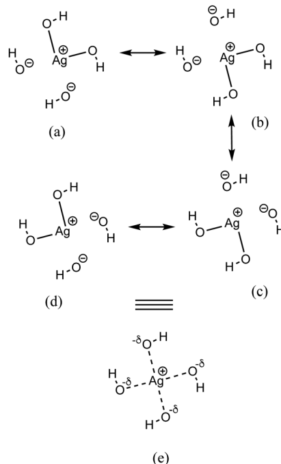
Fig. 7 Resonance structures (a)–(d) and resonance hybrid (e) of the AgO_4H_4^- cluster.
