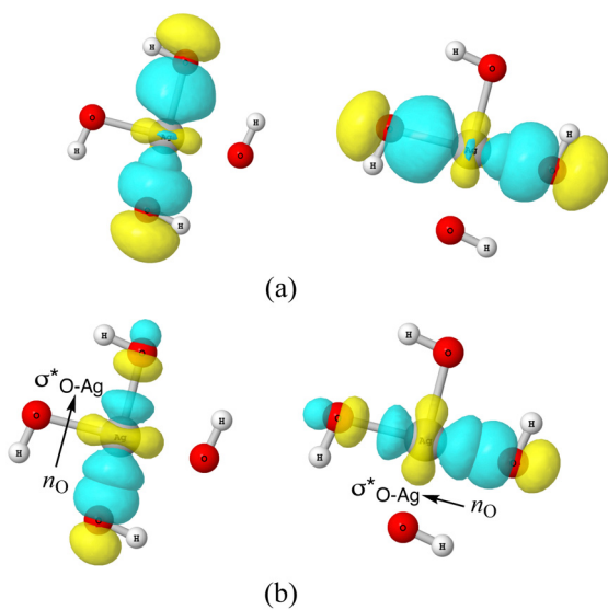
Fig. 6 (a) 3-d surface views of leading 3c/4e Lewis-type NBOs in AgO_4H_4^- cluster (b) lone-pair NBO of O ( n_O ) and empty \sigma^* NBO of Ag-O donor-acceptor pairs in AgO_4H_4^- cluster.
