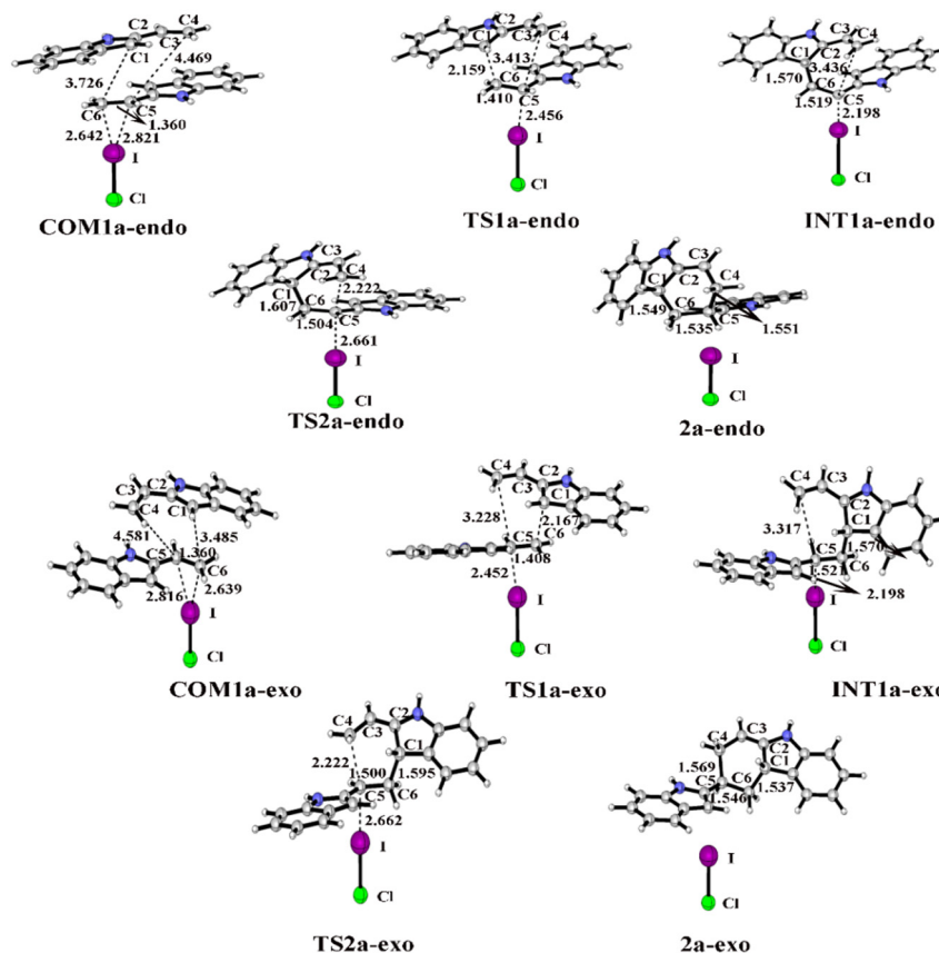
Fig. 5 Optimized geometries and key bond lengths (in Å) along the IRC pathway of I \cdots \pi halogen bond catalysis via ICl activation on the ethenyl of 2-vinylindole.
