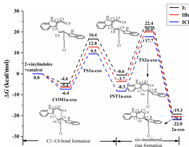
Fig. 7 Gibbs free energy curves of the exo pathway via I \cdots \pi halogen bond catalysis on the ethenyl of 2-vinylindole (mode A).
