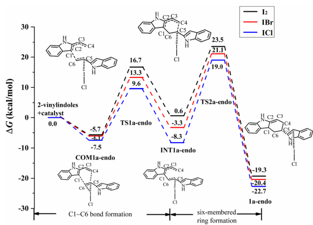
Fig. 6 Gibbs free energy curves of the endo pathway via I...π halogen bond catalysis on the ethenyl of 2-vinylindole (mode A).
