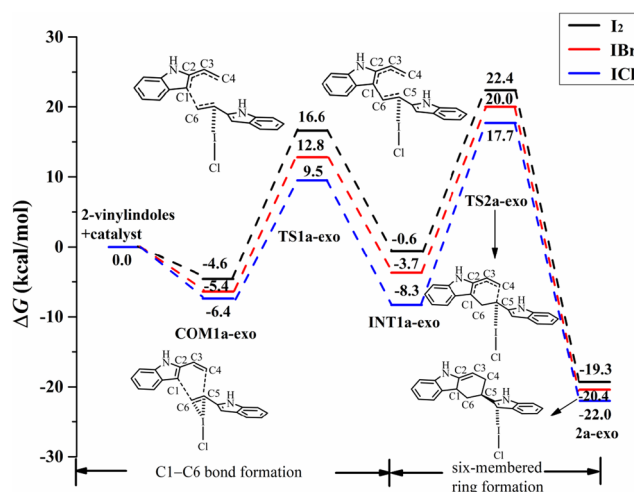
Fig. 7 Gibbs free energy curves of the exo pathway via I...π halogen bond catalysis on the ethenyl of 2-vinylindole (mode A).
