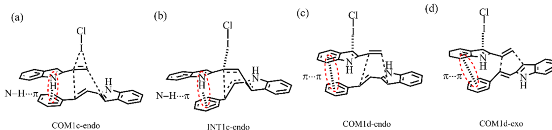
Fig. 13 Structures of COM1c-endo, INT1c-endo, COM1d-endo, COM1d-exo.
