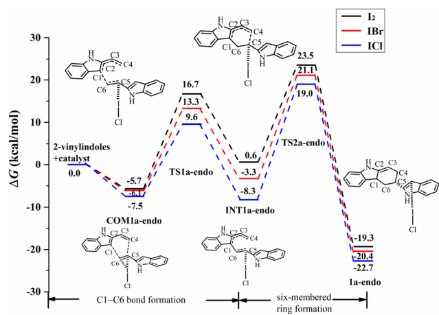
Fig. 6 Gibbs free energy curves of the endo pathway via I \cdots \pi halogen bond catalysis on the ethenyl of 2-vinylindole (mode A).
