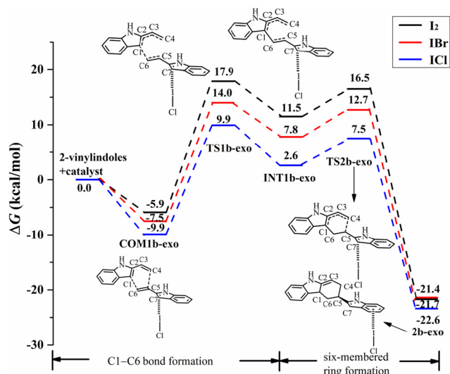
Fig. 10 Gibbs free energy curves of the exo pathway via I... \pi halogen bond catalysis on the five-membered ring of 2-vinylindole (mode B).
