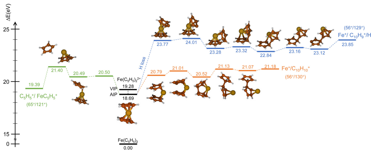
Fig. 4 PES (spin multiplicity – triplet) of the direct mechanisms for the channels \text{C}_5\text{H}_5^+/\text{FeC}_5\text{H}_5^+ (green), \text{Fe}^+/\text{C}_{10}\text{H}_{10}^+ (orange) and \text{Fe}^+/\text{C}_{10}\text{H}_9^+/\text{H} (blue). Relative energies in eV include zero point energy correction ( \Delta E_{\text{ZPE}} ).
