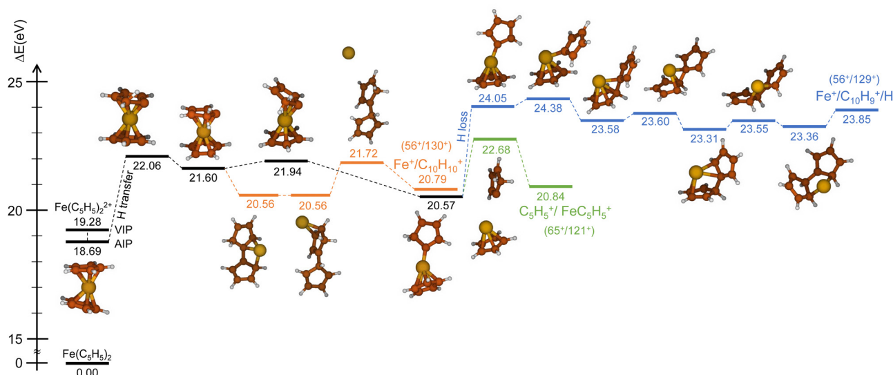
Fig. 5 PES (spin multiplicity – triplet) of the H-transfer mechanisms for the channels \text{C}_5\text{H}_5^+/\text{FeC}_5\text{H}_5^+ (green), \text{Fe}^+/\text{C}_{10}\text{H}_{10}^+ (orange) and \text{Fe}^+/\text{C}_{10}\text{H}_9^+/\text{H} (blue). Relative energies in eV include zero point energy correction ( \Delta E_{\text{ZPE}} ).
