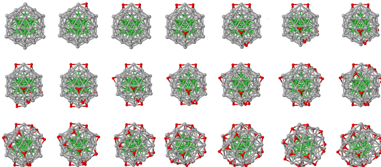
Fig. 1 Putative ground state atomic configurations of \text{Ni}_{13}@Ag_{42}O_m with m = 1 to 20.
