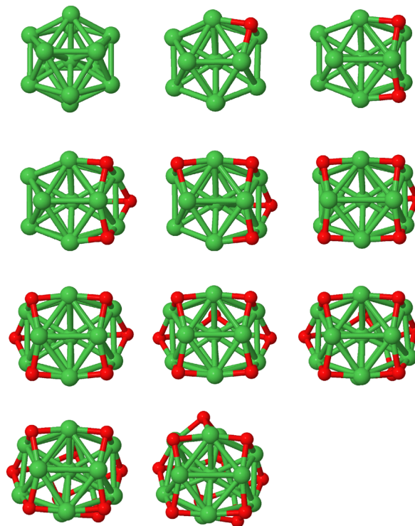
Fig. 2 Putative ground state atomic configurations of \text{Ni}_{13}O_m with m = 1 to 10.
